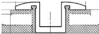
Figure 1 : Laminatklemme ECO 6
